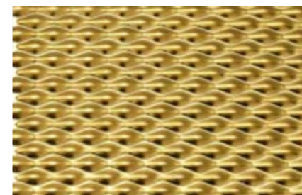
M79
