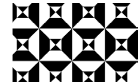
M42
